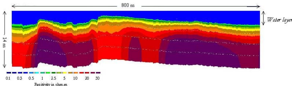
Inversed Resistivity section (3000 data points in 10 minutes)
